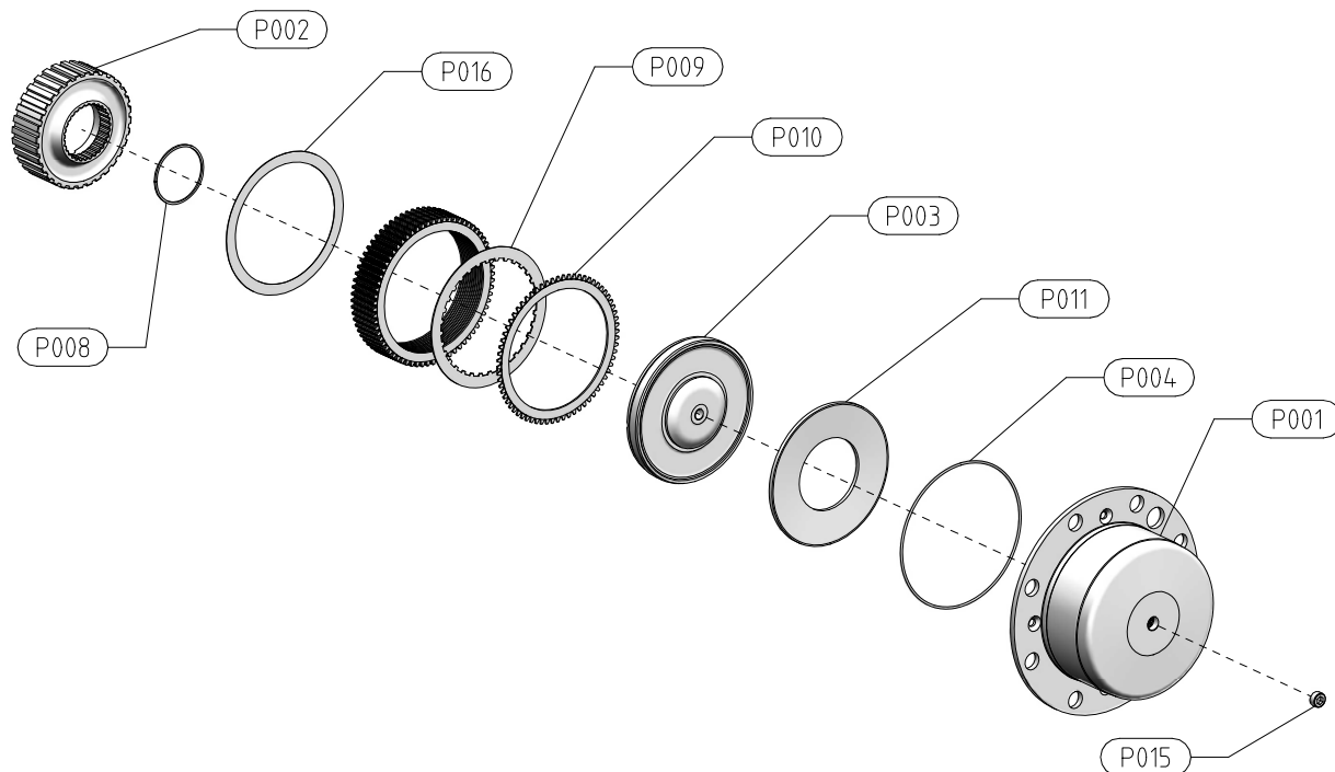
FIG 7. P000, BRAKE KIT, K004312200
