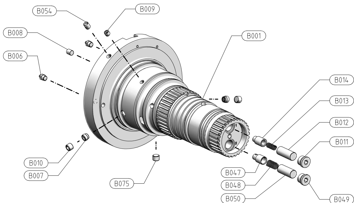
FIG 2. B000, SHAFT ASSEMBLY, K001254413
