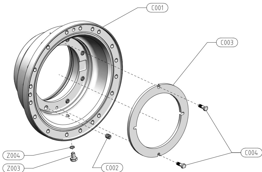
FIG 3. C000, REAR COVER ASSEMBLY, K004323416
