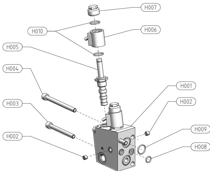
FIG 6. H000, VALVE BLOCK ASSEMBLY, K003920201
