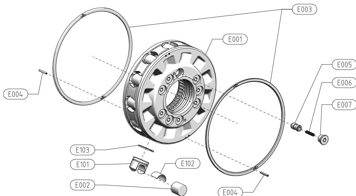
FIG 5. E000, CYLINDER BLOCK ASSEMBLY, K001125100
