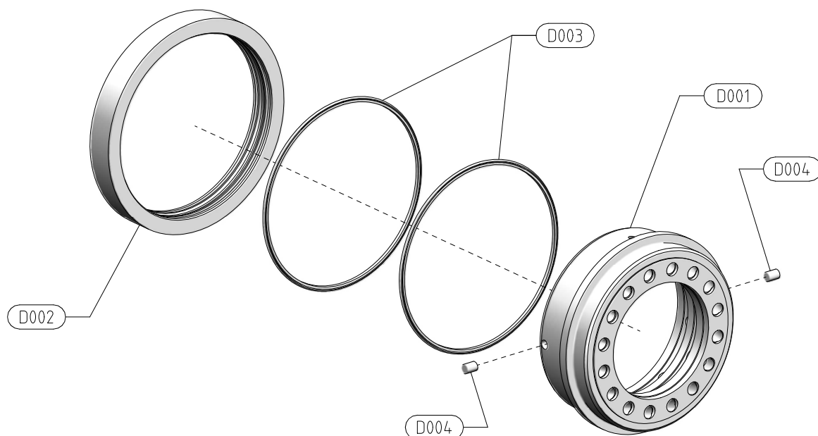
FIG 4. D000, DISTRIBUTION VALVE ASSEMBLY, K003114003
